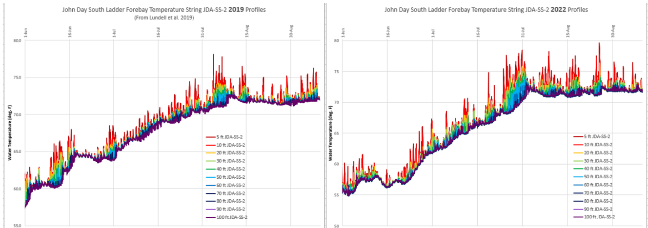
Figure 2: JDA-SS-2 temperatures from June 1 to September 15 in 2019 and 2022. Data shows similar trends in each year.
