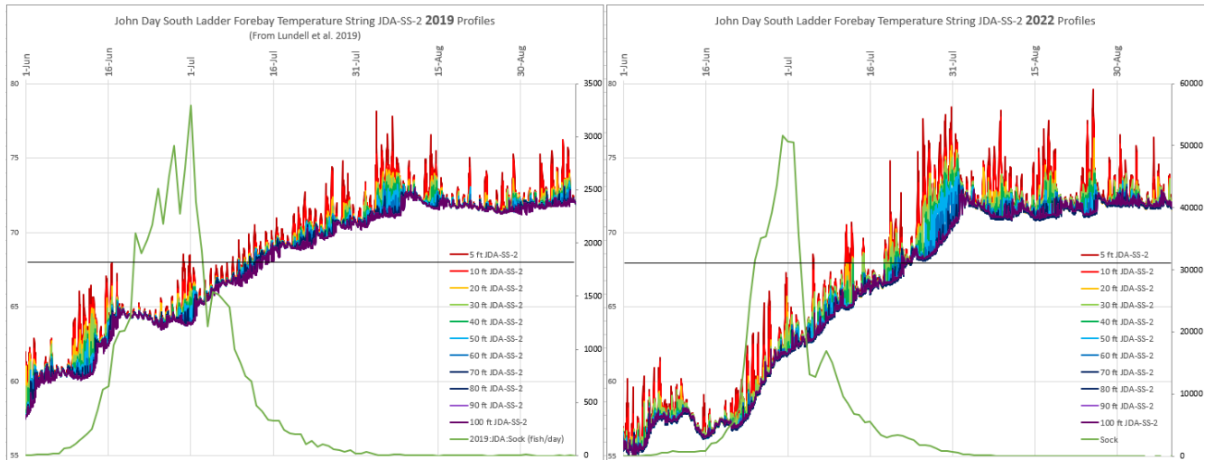
Figure 3: Forebay temperatures (deg. F; left axis) and sockeye passage (fish/day; right axis) for the south fish ladder at John Day Dam in 2019 and 2022.
