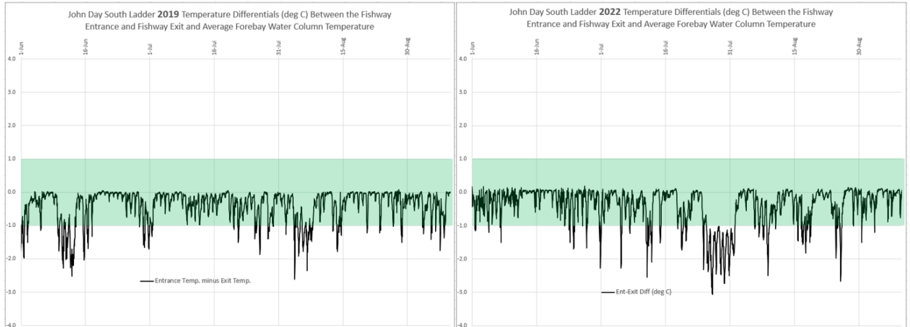
Figure 1: Temperature differentials between the entrance and exits at John Day Dam SFL from June 1 to September 15 in 2019 and 2022.
